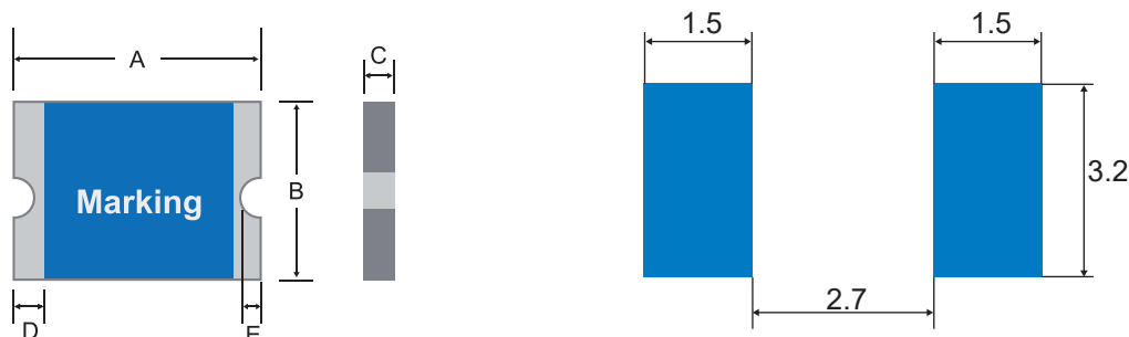
Recommended Pad layout
